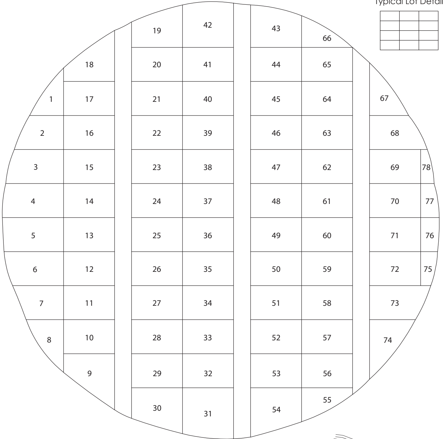
Typical Lot Detail
